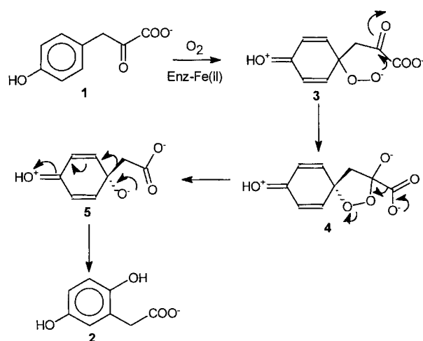
Scheme 1. Proposed HPPD mechanism by Witkop.
