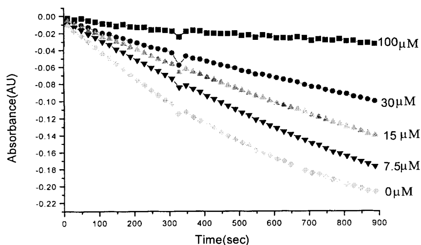
Figure 2. Time-course of the reaction of HPPD and 4-hydroxyphenylpyruvate (35 \mu\text{M} ) with varying concentrations of 14a (100, 30, 15, 7.5, and 0 \mu\text{M} ). The protein concentration in the assay was 1 mg/mL.
