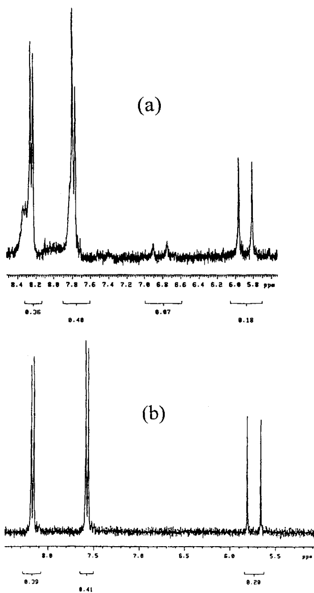
Figure 1. ^1H NMR spectra (300 MHz) of 14b in (a) acetone- d_6 (b) D_2O . The more upfield doublet at 5.88 ppm in (a) was assigned to \beta\text{-H} of 14b with J_{H-F}=44.7 Hz and the small doublet at 6.83 ppm was assigned to \beta\text{-H} of keto form of 14b with J_{H-F}=47.1 Hz.
