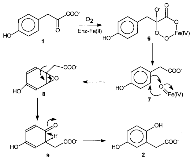
Scheme 2. Proposed HPPD mechanism by Hamilton.
