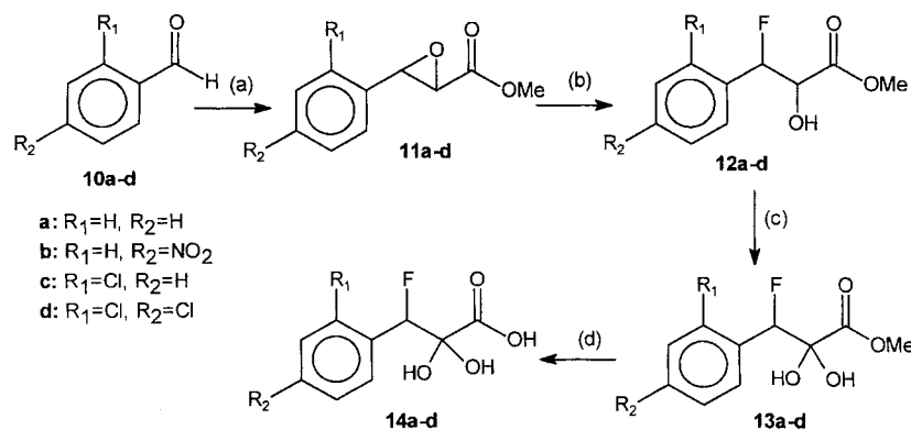
Scheme 3. Synthesis of compounds 14a–d . (a) ClCH_2CO_2Me , NaOMe , MeOH ; (b) HF/pyridine , CH_2Cl_2 ; (c) Jones reagent, acetone; (d) H_2O , i\text{-}PrOH , NaHCO_3 .
